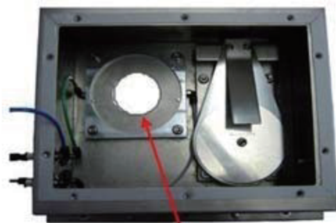
Orifice Plate
